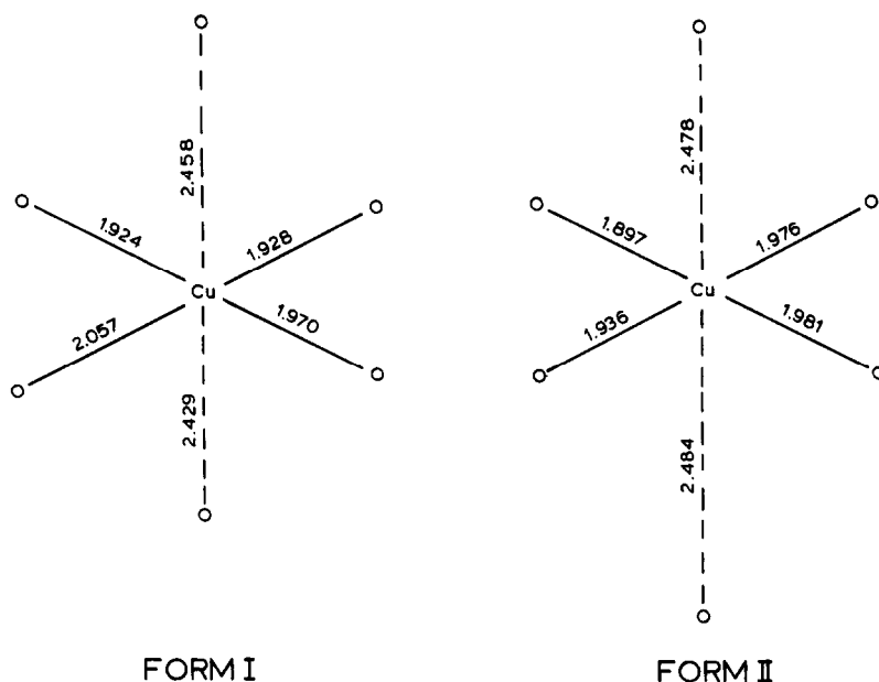
Fig. 5. A schematic representation of the coordination sphere around Cu(II) of dinitratobis(antipyrine)copper(II) isomers [103,104].
