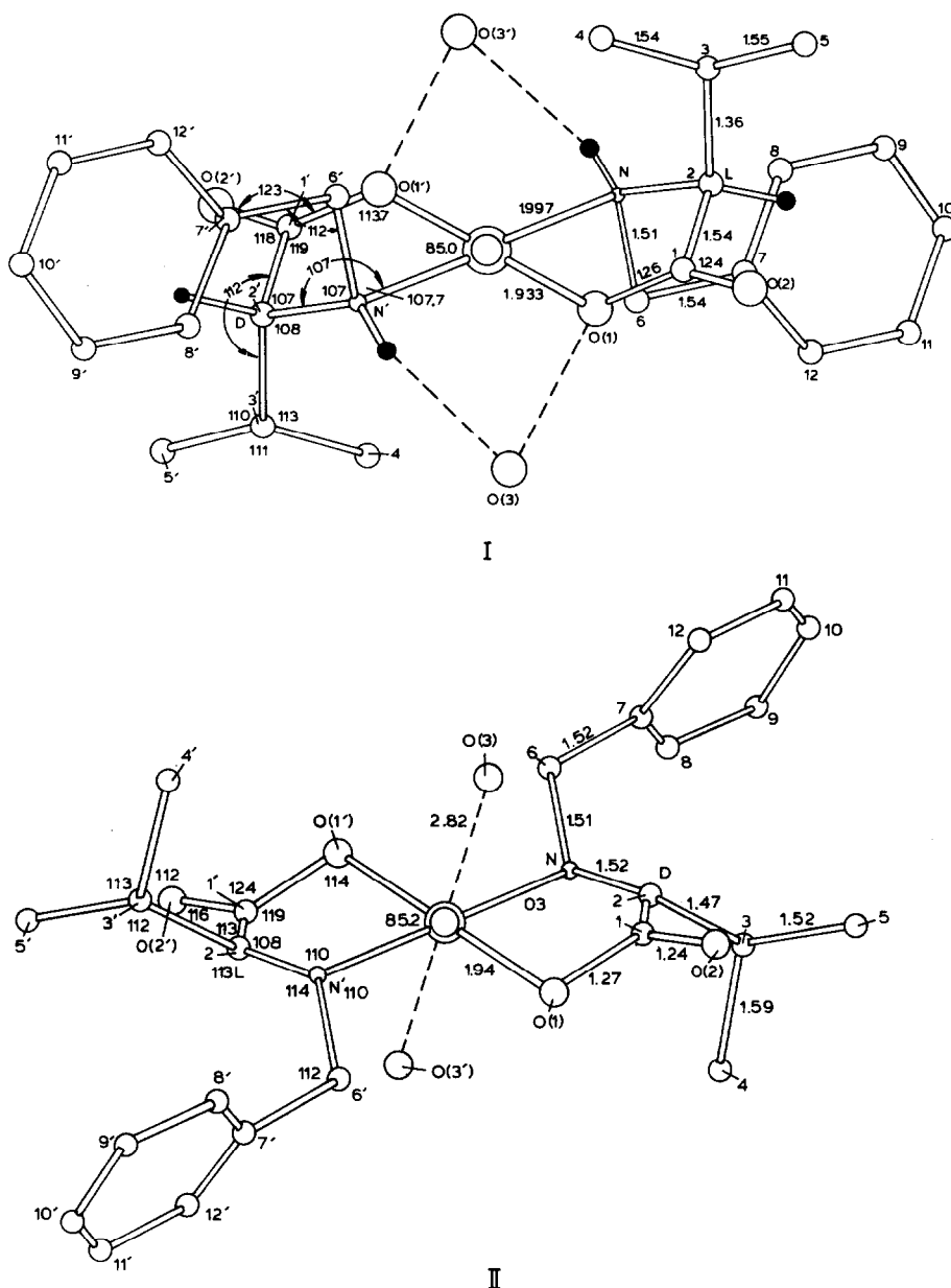
Fig. 3. A schematic view of the crystal structure of the red isomer (I) and blue isomer (II) or ( N -benzyl-L-valinato)( N -benzyl-D-valinato) copper(II) dihydrate [71].
